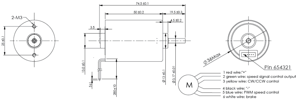
B3650M-S01 (12V)
