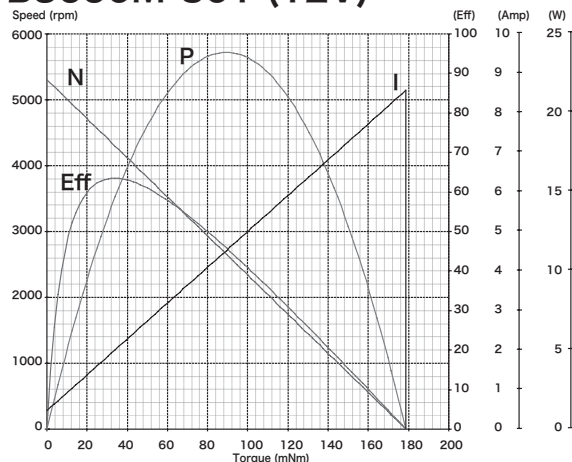
B3650M-S01 (12V)
